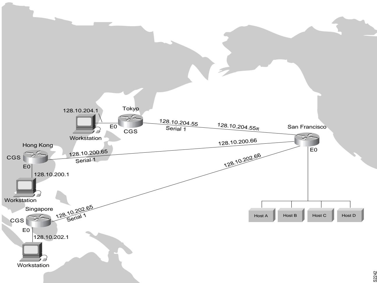
Figure 15-1 DDR internetwork topology.
