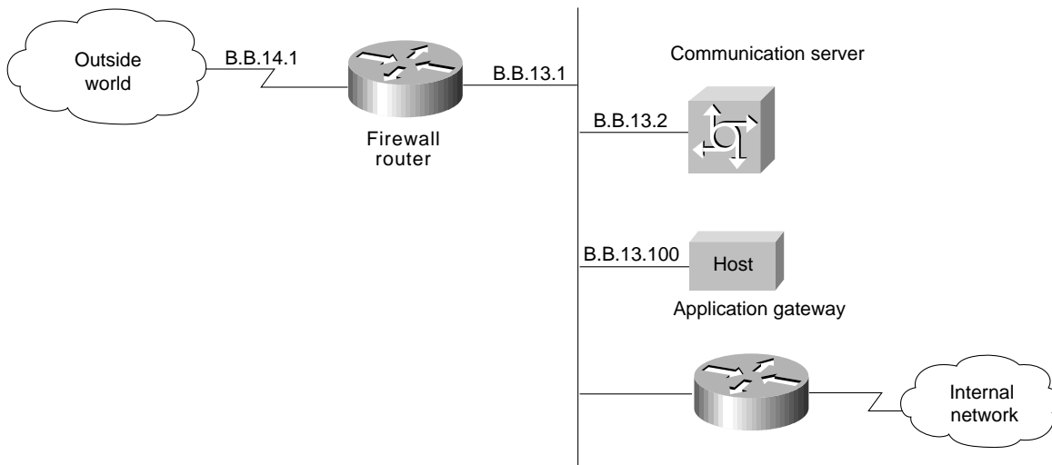
Figure 16-2 Controlling traffic flow via the firewall router.
