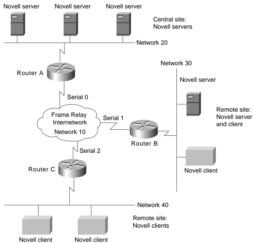
Figure 18-1 Large-scale Novell IPX internetwork.
